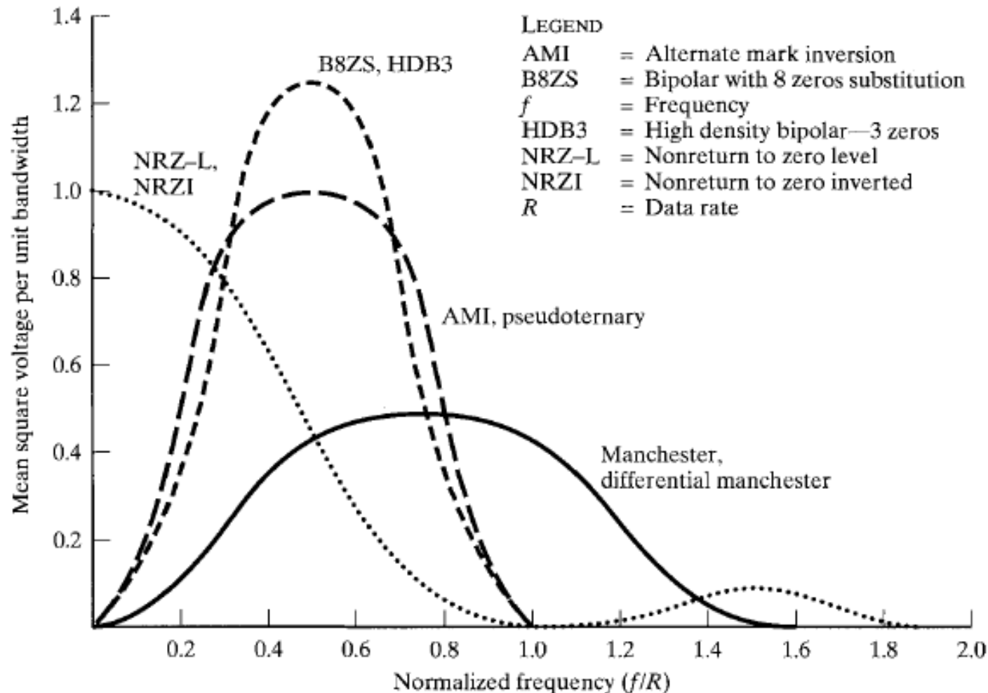
FIGURE 4.3 Spectral density of various signal encoding schemes.
